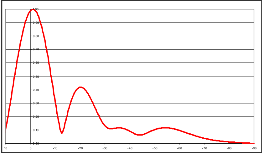
4 Bay Elevation pattern 10 to -90 degrees
